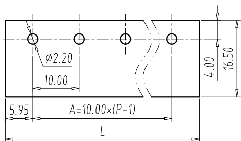
PCB LAYOUT S=5:4
