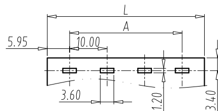
PCB LAYOUT S=1.5:1
