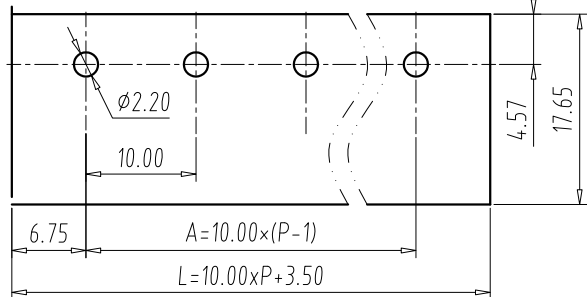
PCB LAYOUT S=1.5:1
