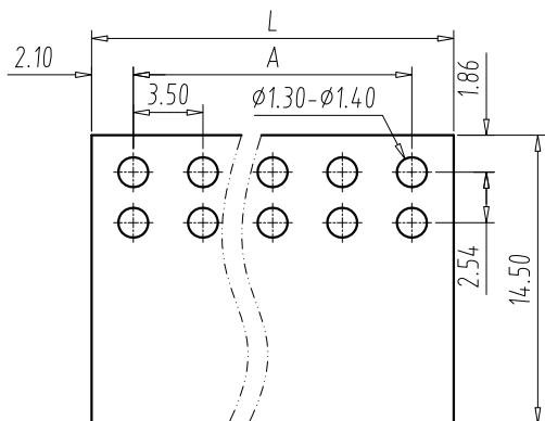
PCB LAYOUT S=2.5:1
