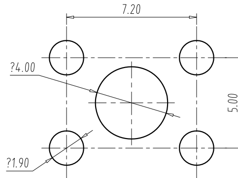
PCB 孔位尺寸 (PCB Hole Dimension)
