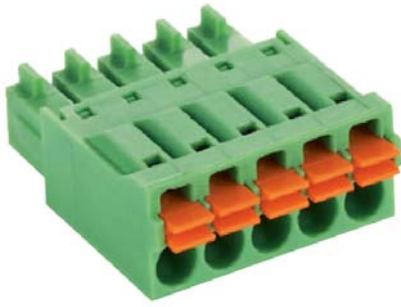
■ 图示(Pic. shown) : TLPS-107-05P-G12
