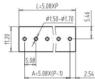
PCB LAYOUT S=1:1
