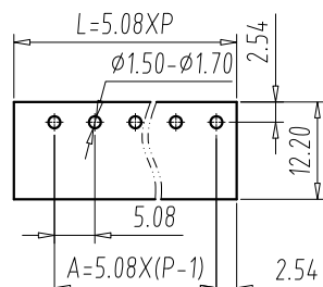
PCB LAYOUT S=1:1
